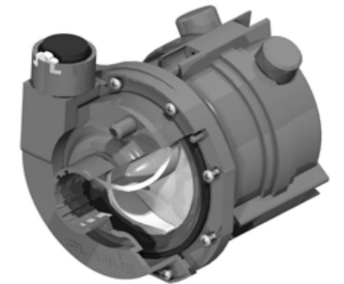
POMPA MACERATRICE BREVETTATA PATENTED INTEGRATED MACERATOR PUMP
